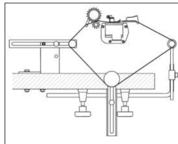
■ RT-1 ゴム張り装置 (手動式) DX, FX(PSF, PMD, PLは除く), RX (RX-P, PLKのみ) RT-1 Elastic expander device ( manual operation ) DX, FX (except for PSF, PMD, PL), RX ( Only for RX-P, PLK ) RT-1 EXPANDIDOR DE ELASTICO DX, FX, RX 松紧带撑开装置 (DX,FX, 除PSF, PMD, PL, RX-P, PLK)
