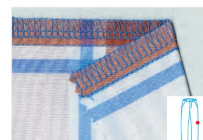
Six threads sewing P15
