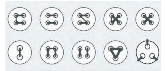
Button attaching stitch P32/P35
