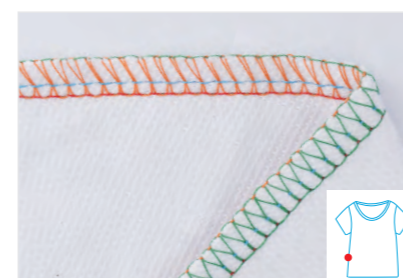
Four threads stitch P15
